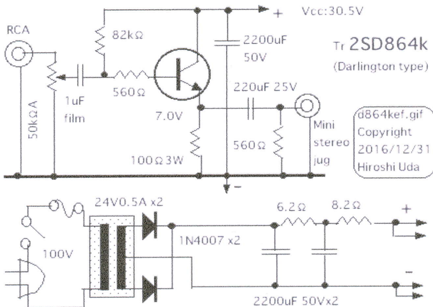
Fig. 2SD864k emitter follower Headphone amp.
