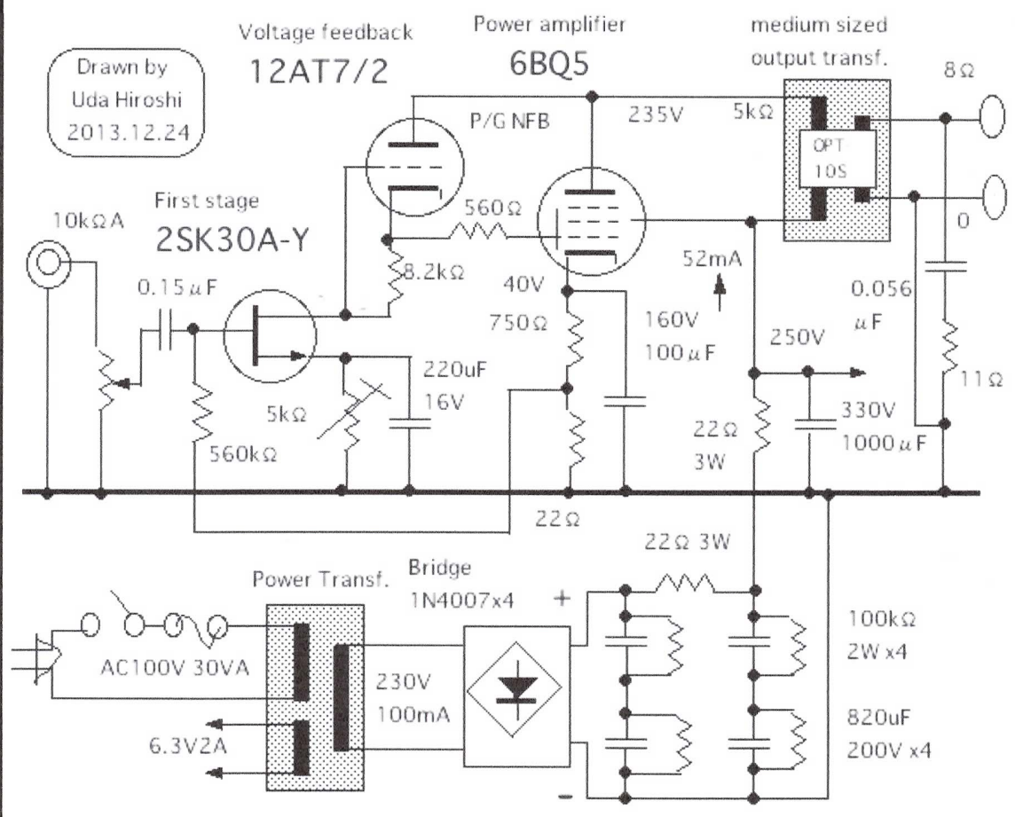
Fig Schematic of 6BQ5 STC amp.
