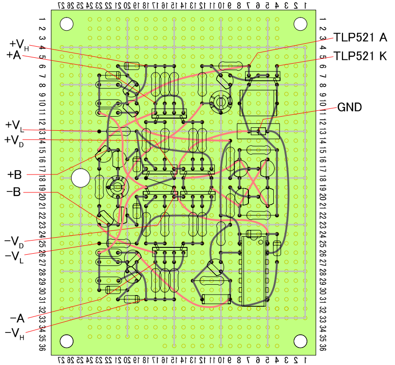
Bottom view
